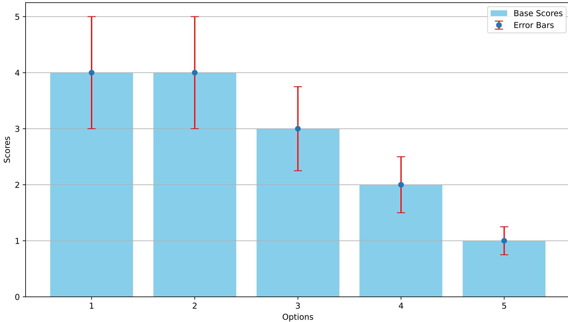
Combined Result Sensitivity Analysis for Acquisition
